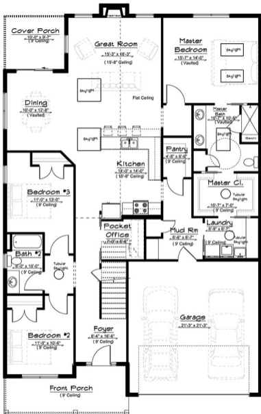
floorplan
