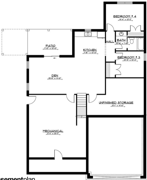
basement plan
